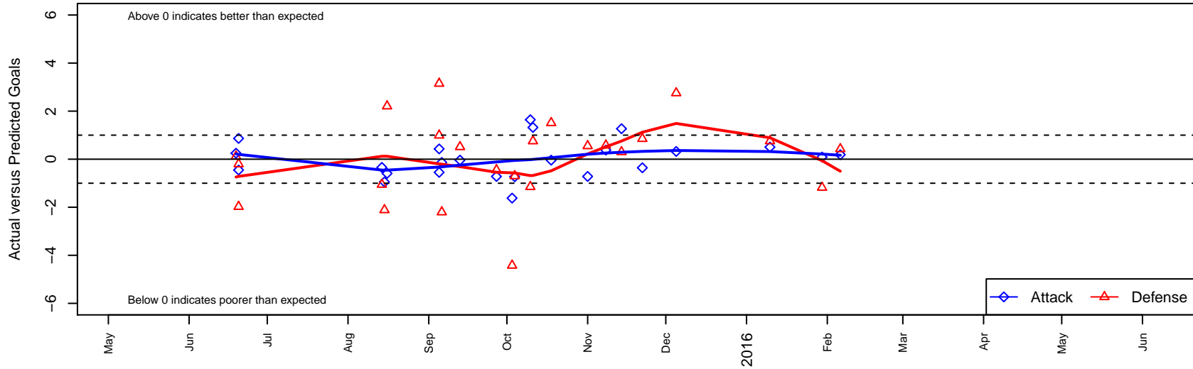
ISC Gunners B B99 Dots are actual minus expected GF (blue circles) and GA (red triangles). Blue line is smoothed change in attack strength. Red is smoothed change in defense strength.
